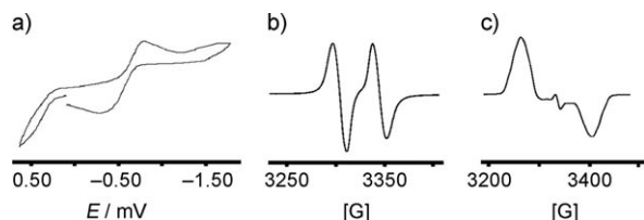
Figure 2. a) Cyclic voltammogram of a THF solution of 5 (0.1 M n BuNPF 6 as electrolyte, scan rate 100 mV s −1 , potential versus Fc + /Fc); b) EPR spectrum (9.3305 GHz) of 5 + in a fluorobenzene solution at 298 K; c) EPR spectrum of 5 + in a fluorobenzene frozen solution at 100 K.
